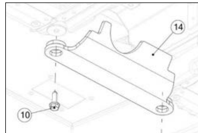
SKI TUNNEL TERRE / Gravel tunnel guard
